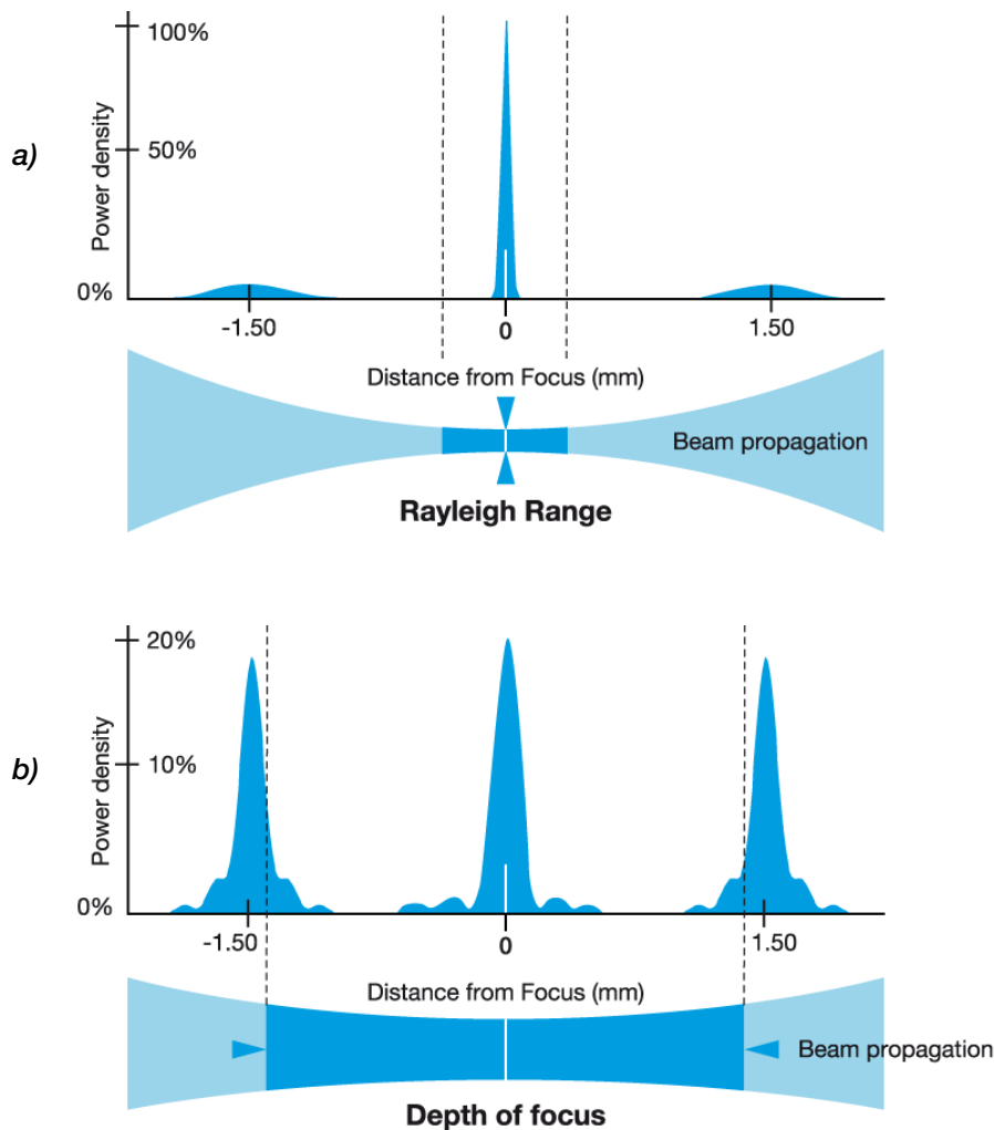
Fig. 3: Micro lines (a) exhibit a high power density at the focus, but line width increases and power density decreases considerably outside this point. Macro lines (b) have a lower power density but an extended depth of focus (approx. 7-40 times larger).
