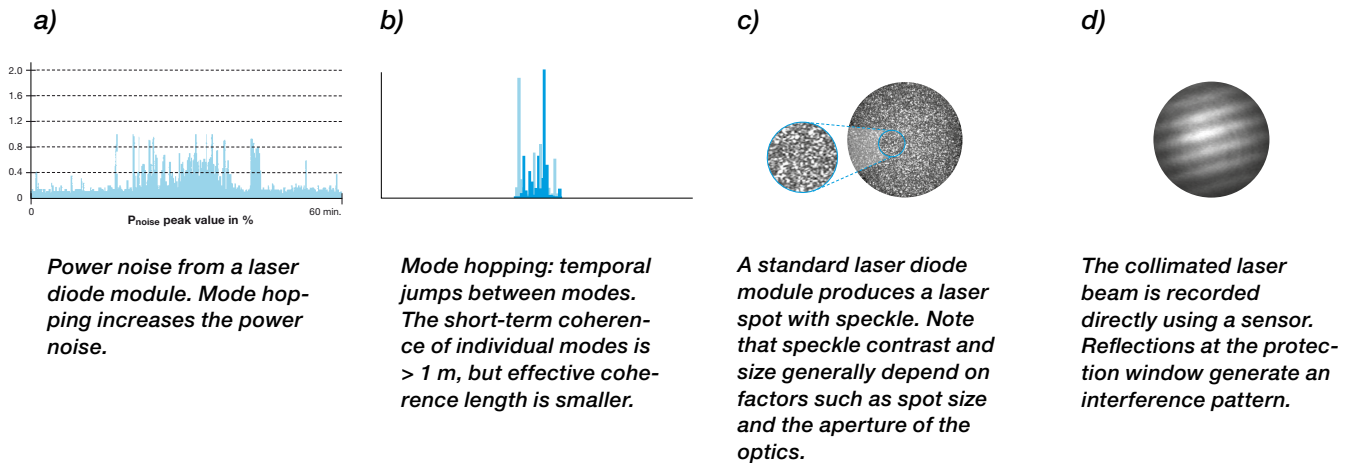
Fig. 5: Characteristics of a standard laser diode beam source. High noise, mode hopping, laser speckle and unwanted interference can constrain the optical resolution.
