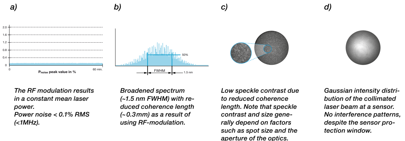
Fig. 6: Advantages of the low noise laser diode beam source with lower noise a), spectral broadening b), reduced laser speckle c) and less interference d).
