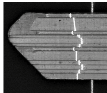
Fig. 2b: Image obtained from the camera. The relative displacement of the laser line provides information about the object height at that point.
