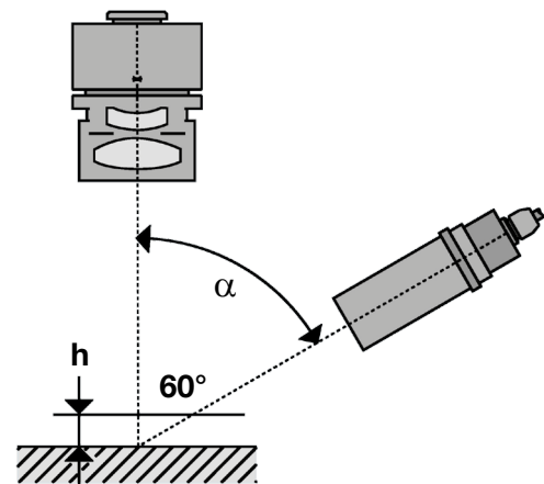
Fig. 2a: Profiling an object with laser triangulation.
