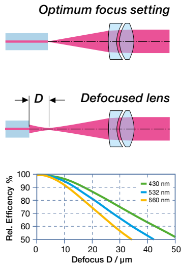
Fig. 2: Axial displacement or defocus: Coupling efficiency with defocused lens, for several wavelengths in the visual range and a fiber NA of 0.1.
