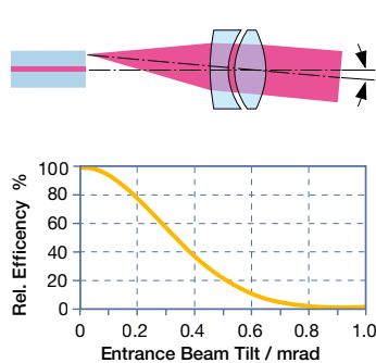
Fig. 3: Lateral adjustment of the mode field and laser spot: Coupling efficiencies for inclined beam propagation. The lateral displacement at the fiber entrance is due to an angular misalignment of the beam. The plot shows an example for wavelength 405 nm, fiber NA_e^2 0.1 and focal length 5mm.
