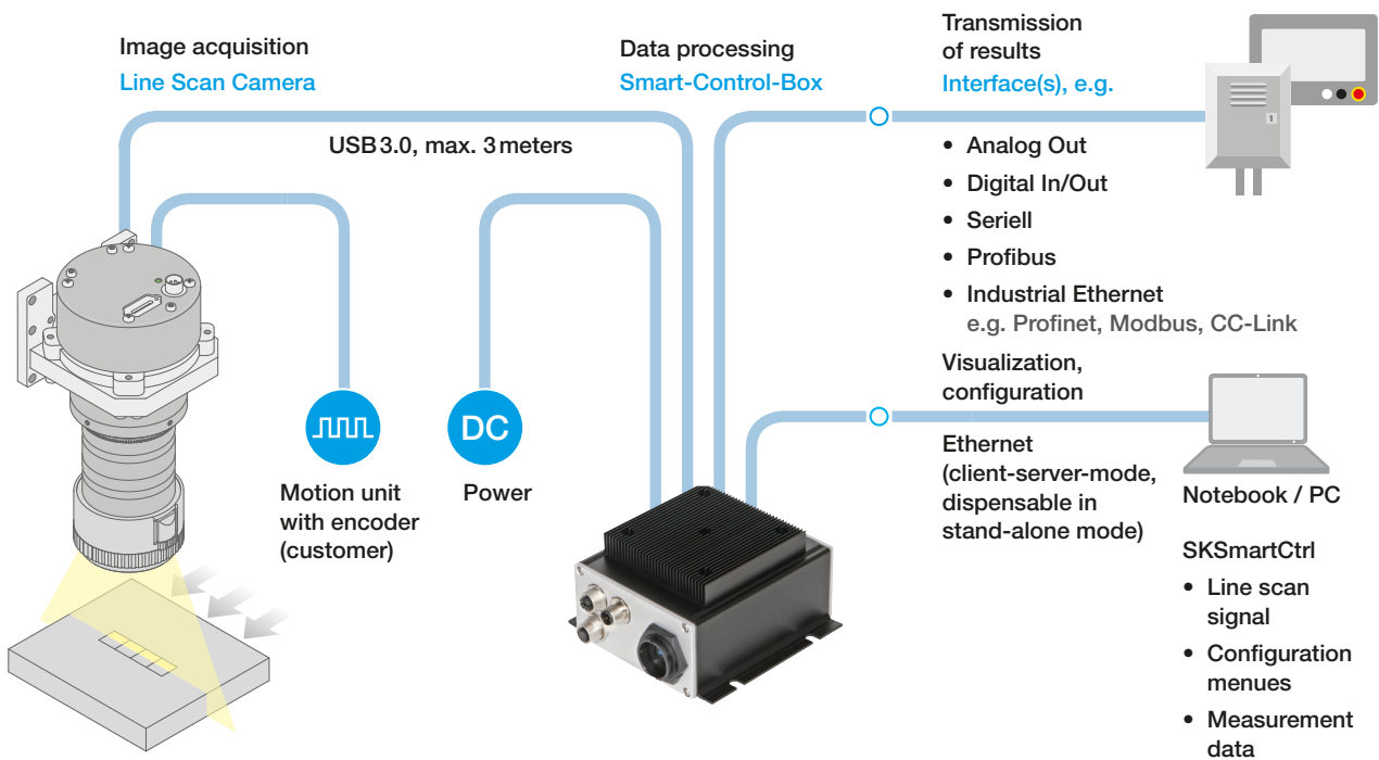
Fig. 2: System components of a smart line scan measurement system. The line scan camera uses the encoder signals of the motion unit for synchronization. The line scans are transferred to the Smart Control Box via a USB 3.0 connection for evaluation. The Smart Control Box operates either in client-server mode, or stand-alone. In stand-alone mode, only a temporary connection to a control computer is required for configuration and set up.
