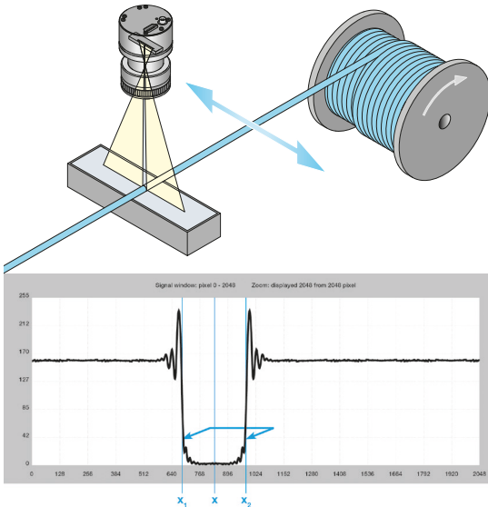
Fig. 3: Spooling inspection of a reel. The light is blocked by the cable, creating a shadow on the sensor. The position of the cable is given by the edges of the shadow. The position measurement is used to check for the correct lateral pendulum movement during spooling.
